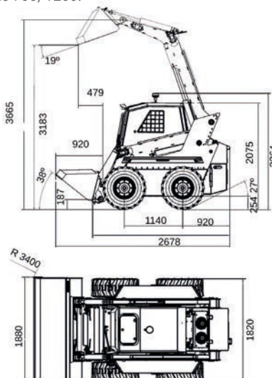
Dimensiones Elise 900/1200:
